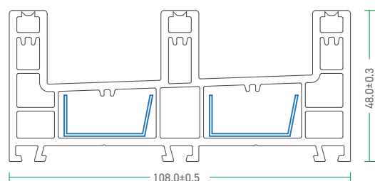
92 - 3SF - C 92 - 3.0 Track Sliding Frame 108
