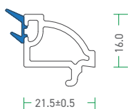
92 - GBS - A 92 - Glazing Bead Sliding 4-8
