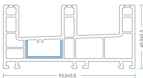
81 - 3SF - B 81 - 3.0 Track Sliding Frame
