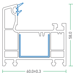
60 - CFM - B 60 - Casement Frame - Medium
