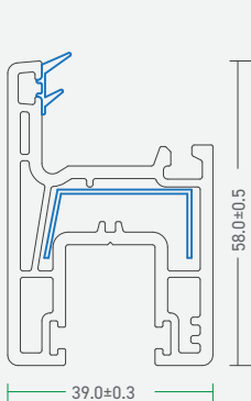
92 - SSS - C 92 - Sliding Sash - Small
