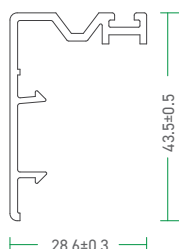
92 - SWSC - A 92 - Sliding Window Sash Cover
