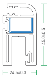
92 - MWS - C 92 & 81 Mesh Window Sash
