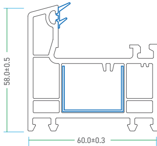
60 - CFM - C 60 - Casement Frame - Medium
