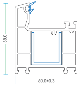
60 - CFB - C 60 - Casement Frame - Big
