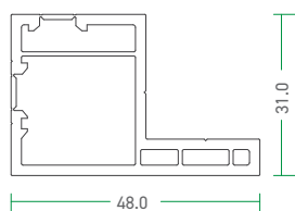
31 - GAT - B Grill Add on track
