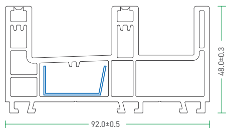
92 - 2.5SF - C 92 - 2.5 Track Sliding Frame
