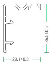
81 - SSC - A 81 - Sliding Sash Cover
