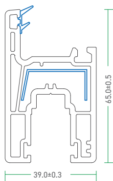
92 - SSM - C 92 - Sliding Sash - Medium
