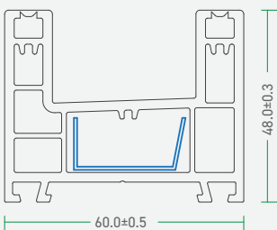
92 - 2SF - C 92 - 2.0 Track Sliding Frame 60
