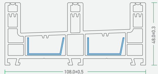
92 - 3SF - C 92 - 3.0 Track Sliding Frame 108
