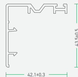
92 - SDSC - A 92 - Sliding Door Sash Cover
