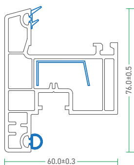
60 - OWS - B 60 - Outward Window Sash
