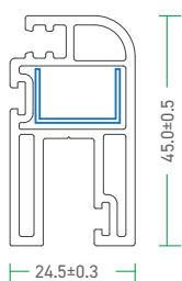
92 - MWS - A 92 & 81 Mesh Window Sash
