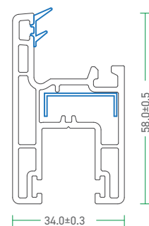
81 - WSS - A 81 - Window Sash - Small
