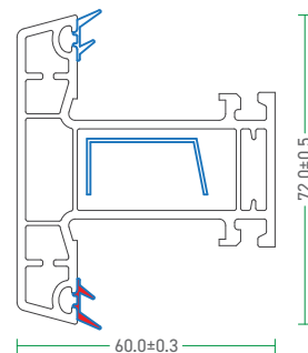
60 - CM - B 60 - Casement Mullion
