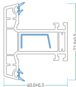
60 - CM - C 60 - Casement Mullion
