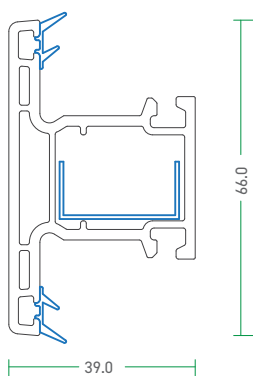
92 - SSM - B 92 - Sliding Sash Mullion
