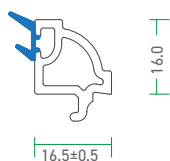
81 - GBSL - A 81 & 92 - Glazing Bead 4-8 & 10-12
