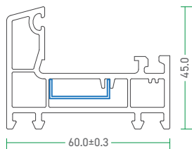
60 - CFS - B 60 - Casement Frame - Small
