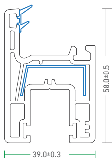
92 - SSS - C 92 - Sliding Sash - Small
