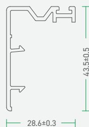
92 - SWSC - A 92 - Sliding Window Sash Cover
