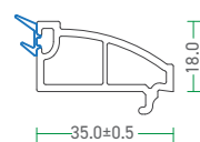
60 - SGB - A 60 - Single Glazing Bead
