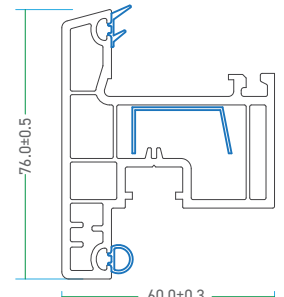
60 - OWS - C 60 - Outward Window Sash
