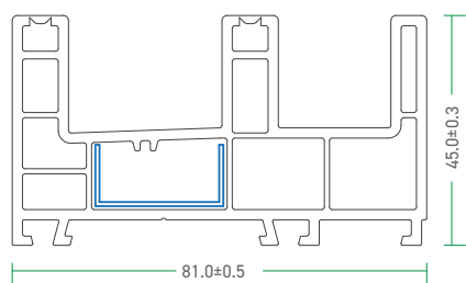
81 - 2.5SF - B 81 - 2.5 Track Sliding Frame
